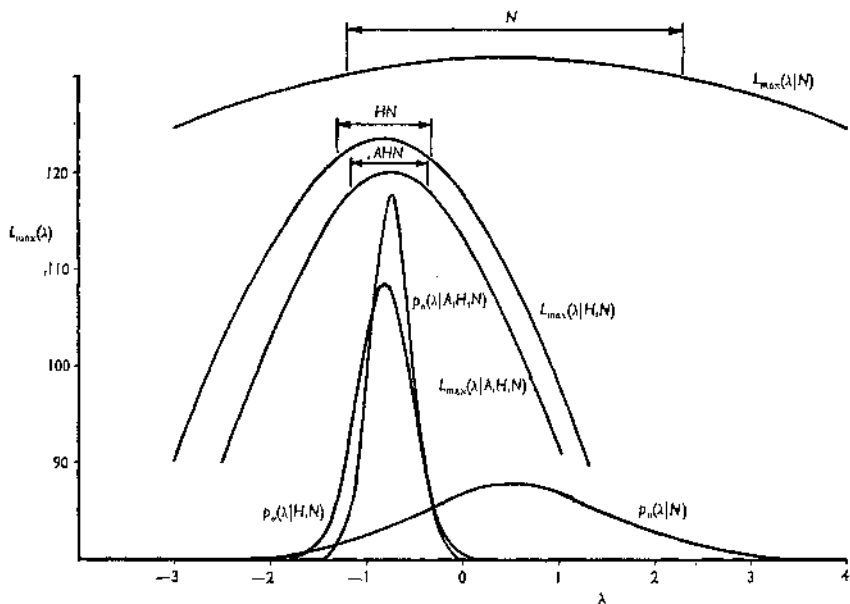
FIG. 6. Biological data. Functions L_{\max}(\lambda) and p_{\lambda}(\lambda) under different models. A : additivity. H : homogeneity of variance. N : normality. Arrows N , HN , AHN show approximate 95 per cent confidence intervals for \lambda .
